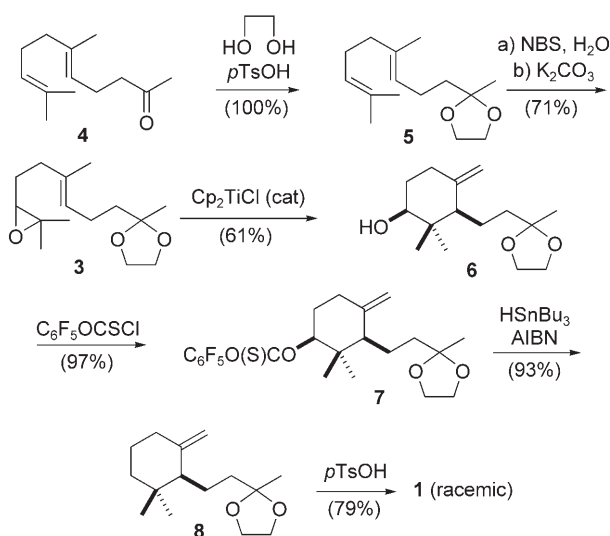
Scheme 2. Synthesis of racemic \alpha -ambrinol ( 1 ).
