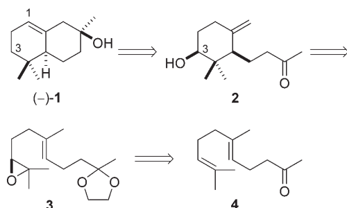
Scheme 1. Retrosynthetic analysis for (–)- 1 .
