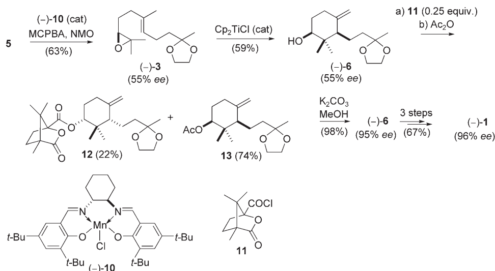
Scheme 4. Enantioselective synthesis of (-) - 1 .
