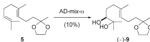
Scheme 3. Asymmetric dihydroxylation of 5 employing AD-mix- \alpha .
