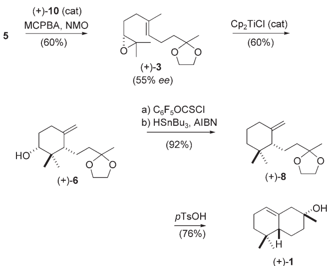
Scheme 5. Enantioselective synthesis of (+) - 1 .
